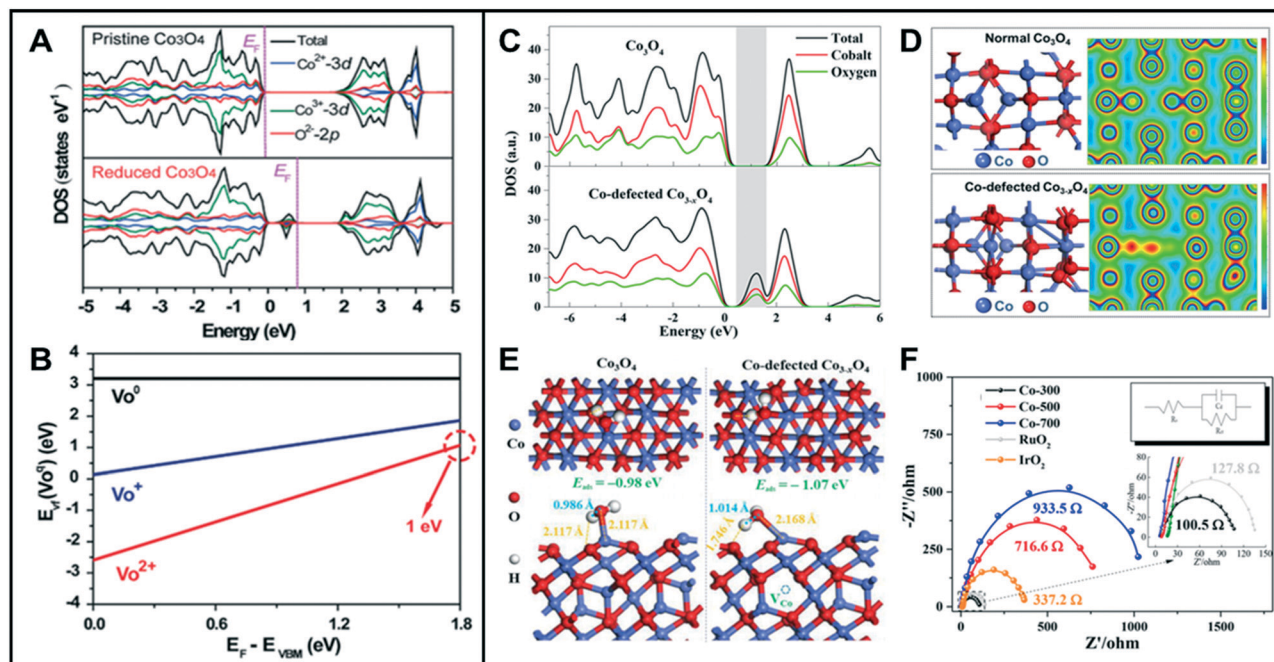
Fig. 3 (A) TDOS and PDOS of pristine Co 3 O 4 and reduced Co 3 O 4 with oxygen vacancies. (B) Calculated formation energies for the reduced Co 3 O 4 . V O 2+ , V O + , and V O 0 denote that the gap state is empty, occupied by one electron, and occupied by two electrons, respectively. Reproduced with permission from ref. 26. Copyright 2014 Wiley-VCH. (C) TDOS and PDOS for Co 3 O 4 and Co-defected Co 3-x O 4 . (D) Optimized cell structures and the corresponding charge density mapping of normal Co 3 O 4 and Co-defected Co 3-x O 4 . (E) Optimized structures of water adsorbed at Co on the (111) surface (top and side views) of Co 3 O 4 (left) and Co 3-x O 4 (right). (F) Electrochemical impedance spectroscopy (EIS) (inset: EIS fitting model; electrolyte resistance R_s , charge-transfer resistance R_{ct} , capacitive reactance C_d ). Reproduced with permission from ref. 3. Copyright 2018 American Chemical Society.
