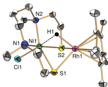
Fig. 1 ORTEP drawing of 2 with ellipsoids set at the 50% probability level. The hydrogen atoms of the ligand X ( N,N' -dimethyl-3,7-diazanonane-1,9-dithiolato) and C 5 Me 5 are omitted for clarity. Selected interatomic distances [Å] and angles [°]: Ni1···Rh1 2.7454(16), Rh1–H1 1.84(9), Ni1–H1 1.96(9), Ni1–S1–Rh1 71.15(7) and Ni1–S2–Rh1 70.65(7) for 2 .
