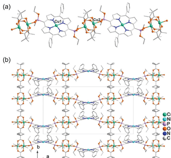
Fig. 9 (a) Linear chain structure of 46 . (b) Zigzag chain structure of 48 . Adapted from ref. 50 and 54.
