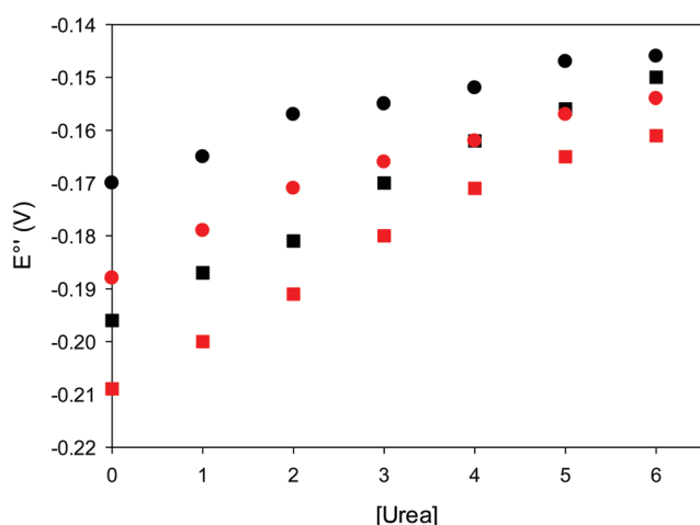
Fig. 7 Urea-induced changes in E^{\circ} for the M80A (circles) and M80AY67A (squares) variants of S. cerevisiae iso-1 cytochrome c at 5^\circ\text{C} (red) and 25^\circ\text{C} (black). Working electrode: polycrystalline gold wire functionalized with 4-mercapto-pyridine. 10 mM phosphate buffer plus 100 mM sodium perchlorate, pH 7.2.
