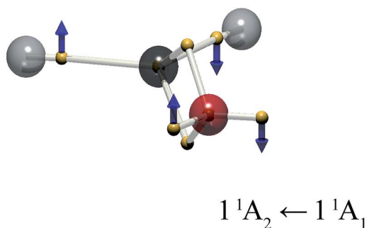
Fig. 4 The electron positions for the mid-point of the vibration, \bar{x} = (\bar{x}_i + \bar{x}_j)/2 , and the displacement vectors x_{fi} for the wavefunction mixed between the 1^1A_1 (ground), and 1^1A_2 , 2^1A_1 and 1^1B_1 excited states of formaldehyde. The vector length is doubled for clarity.
