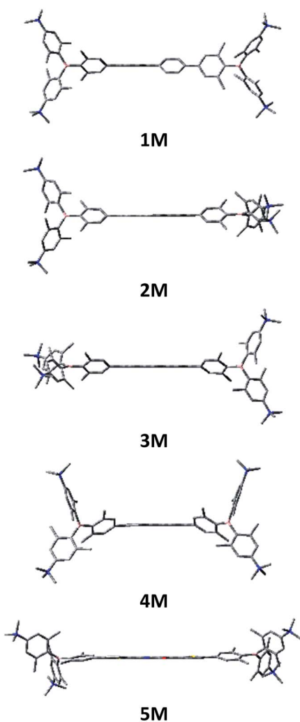
Fig. 8 Side view of the geometries of the DFT-optimized S_0 states of 1M–5M at the B3LYP/6-31G(d) level of theory. Atom colour code: carbon (grey), boron (pink), sulphur (yellow), nitrogen (blue), oxygen (red). Hydrogen atoms are omitted for clarity.
