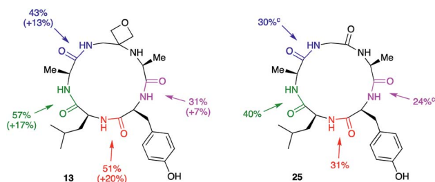
Fig. 5 Macrocyclisation efficiency as a function of location of oxetane relative to forming amide bond. a,b a Reaction conditions: DEPBT (2 equiv.), 1 Pr 2 EtN (2 equiv.), DMF (0.001 M), RT, 24 h. b Average of two runs. c Taken from ref. 12.
