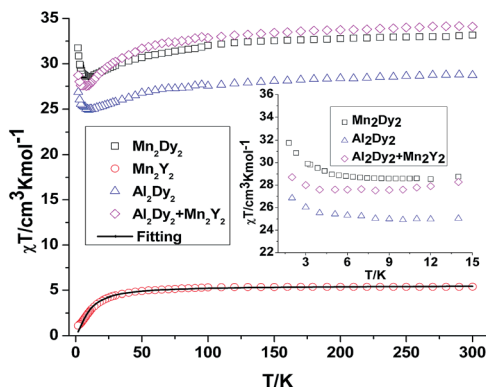
Fig. 3 Temperature dependence of the \chi T product at 300 Oe for 3 \{\text{Mn}_2\text{Dy}_2\} , 4 \{\text{Mn}_2\text{Y}_2\} (the solid line is the best fit to the experimental data for 4). The comparison curves (inset) of \{\text{Mn}_2\text{Dy}_2\} and \{\text{Al}_2\text{Dy}_2\} + \{\text{Mn}_2\text{Y}_2\} along with the curves of 4 \{\text{Mn}_2\text{Y}_2\} and 7 \{\text{Al}_2\text{Dy}_2\} enlarged in the region below 15 K.
