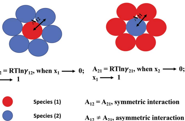
Fig. 1 A cartoon representation of asymmetric interaction in a binary mixture at infinite dilution.
