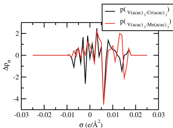
Fig. 4 Sigma profile of metal complexes.
