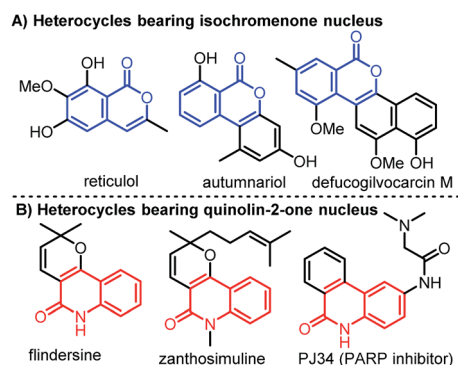
Fig. 1 Biologically active heterocycles bearing isochromenone or quinolinone moiety.
