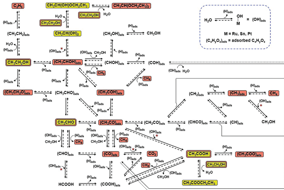
Fig. 17 Ethanol electrochemical reaction pathways on Pt-based catalysts. The reaction steps marked with red stars are those in which \text{OH}_{\text{ads}} are involved and catalytic sites are regenerated due to reaction with \text{OH}_{\text{ads}} . The chemical species highlighted in yellow were observed in this study, and those highlighted in brown were observed in earlier studies that used other analytical techniques. Adapted with permission from ref. 194. Copyright 2011, Wiley-VCH.
