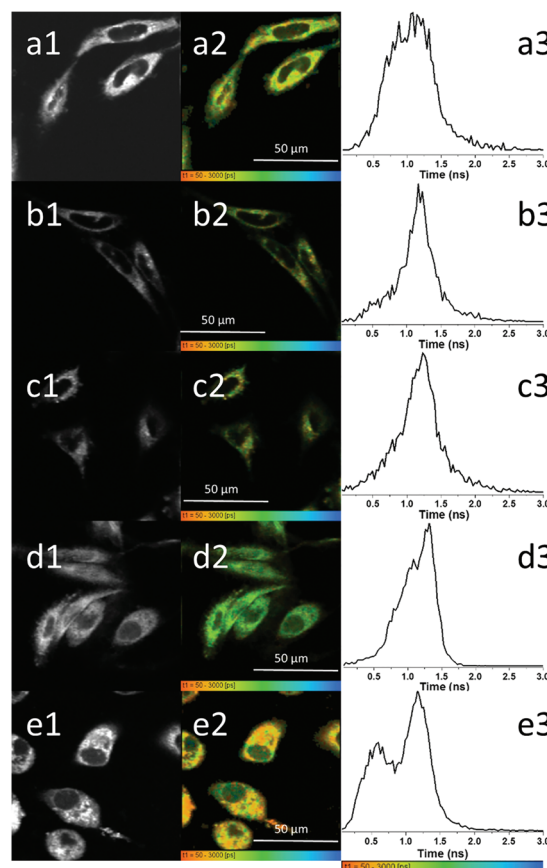
Fig. 4 Two-photon fluorescence imaging including lifetime microscopy mapping of 5-P (100 \mu\text{M} in 0.5 : 99.5% DMSO : RPMI) ( a_{1-2} ; b_{1-2} ; d_{1-2} ) and 5@ \beta -D-glucan (0.5 : 99.5% DMSO : RPMI) ( c_{1-2} ; e_{1-2} ) in HeLa ( a_{1-2} ; b_{1-2} ; c_{1-2} ) and PC-3 cells ( d_{1-2} ; e_{1-2} ) after 15 min incubation. Corresponding fluorescence lifetime distribution curves: a_3 , b_3 , c_3 , d_3 , e_3 ; \lambda_{\text{ex}} = 810 nm. Scale bar: 50 \mu\text{m} . The micrographs show that 5-P and 5@ \beta -D-glucan are capable of penetrating the cell membrane at either 4 ^{\circ}\text{C} ( b_{1-2} ; c_{1-2} ) or at 37 ^{\circ}\text{C} ( a_{1-2} ; d_{1-2} ; e_{1-2} ), although the lower temperature reduces the extent of cellular uptake. Legend colours provide a direct correlation between the lifetime maps a_2 – e_2 and the histograms showing the corresponding lifetimes distribution ( a_3 – e_3 ).
