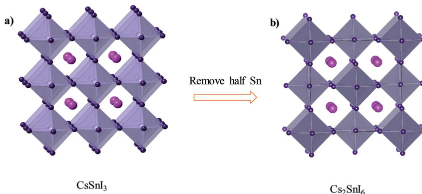
Fig. 8 (a) Crystal structure of \text{CsSnI}_3 . (b) Crystal structure of \text{Cs}_2\text{SnI}_6 . Consulting from ref. 79.
