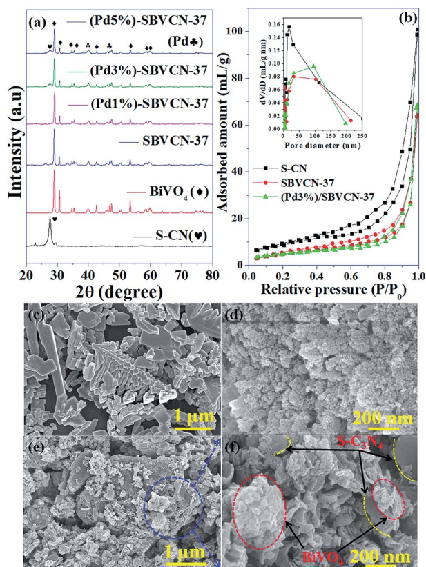
Fig. 1 (a) Powder XRD patterns of all the materials synthesized in this study, (b) N_2 adsorption–desorption isotherms of S-CN, SBVCN-37, and (Pd3%)/SBVCN-37 (inset shows BJH pore size distribution) and FESEM images of (c) BiVO_4 , (d) S-CN, (e) SBVCN-37, and (f) (Pd3%)/SBVCN-37 photocatalyst.
