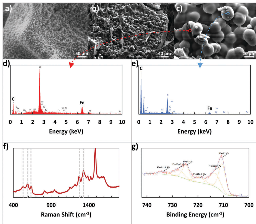
Fig. 2 (a) ESEM image and (b) and (c) SEM images of spherical structures present in dopamine–iron–alginate gel. (d and e) Show EDX analysis of the locations marked in (c), with (d) focusing on the interior of a cracked sphere, and (e) examining the surface of a sphere. (f) Shows a Raman spectrum of dopamine–iron–alginate gel. (g) Shows a high-resolution XPS spectrum of the Fe 2p peaks for iron–alginate gel.
