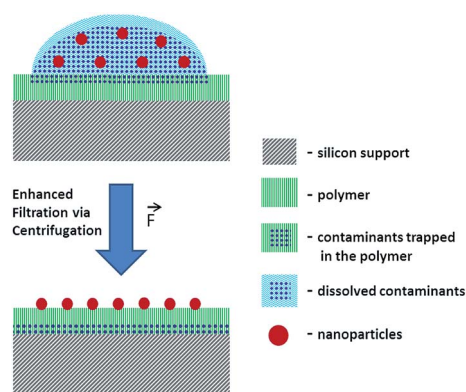
Fig. 1 Sketch of the developed NPs deposition and cleaning concept. After the deposition, the hydrophilicity of the polymer coated silicon wafer allows the penetration of water and solutes into the bottom part of the polymer leaving the clean NPs onto the upper part. This filtration process can be enhanced via centrifugation.
