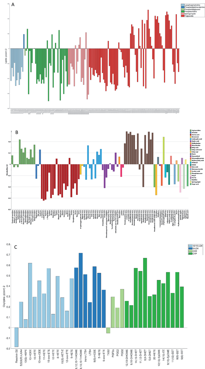
Fig. 5 Second globally joint loading vectors ( p(\text{corr}) ) for the lipids (A), metabolites (B) and oxylipins (C) data sets coloured according to the chemical classes (metabolites and lipids) and biochemical pathways (oxylipins).
