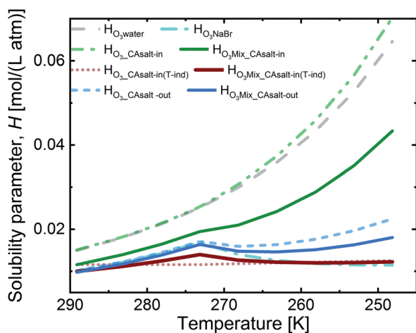
Fig. 4 Calculated ozone solubility in solution fractions and in the mixture (by the volume mixing rule). H_{O_3,i} is Henry's law O_3 solubility in solution (i). Grey dashed line: H_{O_3water} ; cyan dash-dot line: H_{O_3NaBr} ; green dash-dot-dot line: H_{O_3-CA_{salt-in}} , salting-in effect with T dependence of H_{O_3water} ; red dotted line: H_{O_3-CA_{salt-in}(T-ind)} , salting-in effect without T -dependence; blue dashed line: H_{O_3-CA_{salt-out}} , salting-out effect with T dependence of H_{O_3water} ; solid green line: H_{O_3-Mix\_CA_{salt-in}} with H_{O_3-CA_{salt-in}} ; solid red line: H_{O_3Mix\_CA_{salt-in}(T-ind)} with H_{O_3-CA_{salt-in}(T-ind)} ; solid blue line: H_{O_3Mix\_CA_{salt-out}} with H_{O_3-CA_{salt-out}} ; all H_{O_3Mix} contain volume ratio combinations of the H_{O_3-CA} scenarios and H_{O_3NaBr} surface reaction.
