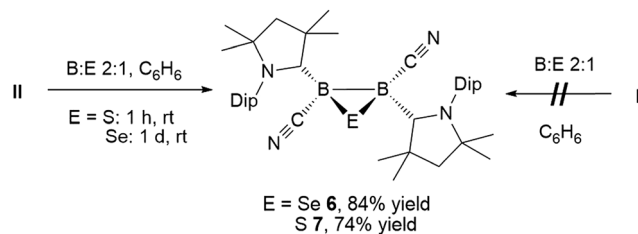
Scheme 5 Direct synthesis of 1,2,3-chalcogenadiboriranes from 11 only.
