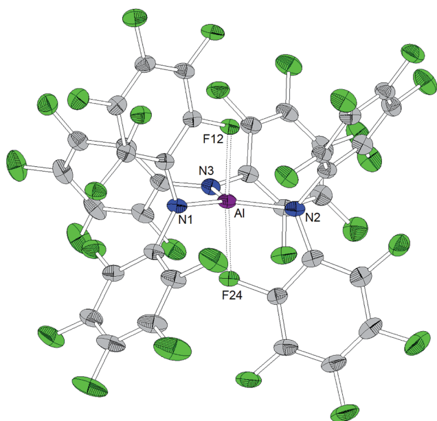
Chart 2 Molecular structure of \text{Al}[\text{N}(\text{C}_6\text{F}_5)_2]_3 (ellipsoids with 30% probability). Selected bond lengths/Å and angles/ ^\circ : Al–N1 1.843(2), Al–N2 1.840(2), Al–N3 1.805(2), \text{Al}\cdots\text{F12} 2.084(1), \text{Al}\cdots\text{F24} 2.060(1), \text{N1–Al–N2} 123.7(1), \text{N2–Al–N3} 116.2(1), \text{N3–Al–N1} 120.09(9), \text{F24–Al–F12} 164.93(6) .
