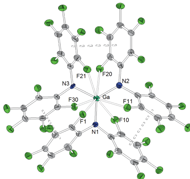
Chart 3 Molecular structure of \text{Ga}[\text{N}(\text{C}_6\text{F}_5)_2]_3 (ellipsoids with 30% probability). Selected bond lengths/Å and angles/ ^\circ : Ga–N1 1.826(5), Ga–N2 1.798(5), Ga–N3 1.848(5), \text{Ga}\cdots\text{F1} 3.032(4), \text{Ga}\cdots\text{F10} 2.981(4), \text{Ga}\cdots\text{F11} 3.096(4), \text{Ga}\cdots\text{F20} 2.994(4), \text{Ga}\cdots\text{F21} 3.102(4), \text{Ga}\cdots\text{F30} 2.914(4), \text{N1–Ga–N2} 122.8(2), \text{N2–Ga–N3} 123.0(2), \text{N3–Ga–N1} 114.3(2).
