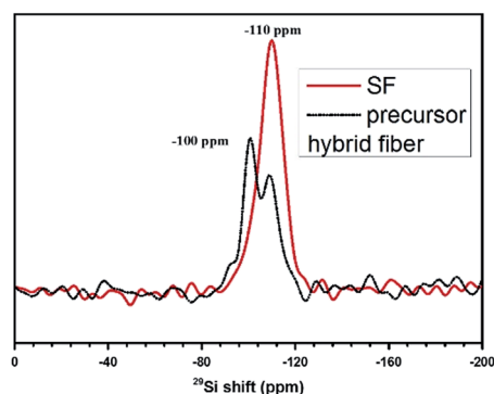
Fig. 3 The ^{29}\text{Si} NMR test of precursor hybrid fiber membrane and SF.
