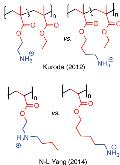
Fig. 14 The length of the spacer arm that connects a cation to the polymer backbone is a key design parameter.
