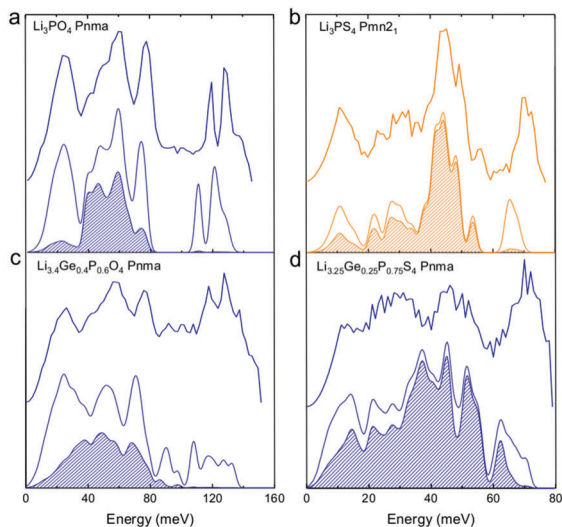
Fig. 2 Measured phonon DOS and computed total and lithium-projected phonon DOS. Experimental phonon DOS collected at 100 K are shown on top while computed phonon DOS at 0 K are shown on the bottom as well as the computed lithium-projected DOS (shaded). (a) \text{Li}_3\text{PO}_4 ( Pnma ) (b) \text{Li}_3\text{PS}_4 ( Pnm2_1 ) (c) \text{Li}_{3.4}\text{Ge}_{0.4}\text{P}_{0.6}\text{O}_4 ( Pnma ) and (d) \text{Li}_{3.25}\text{Ge}_{0.25}\text{P}_{0.75}\text{S}_4 ( Pnma ). The measured phonon DOS data were obtained after background correction, optimizing lower and higher energy cut-off and details can be found in Fig. S4 (ESI † ). The computed DOS were weighted by neutron scattering cross section of the different elements that make up the structures. The details of this procedure can be found in previous work. 67
