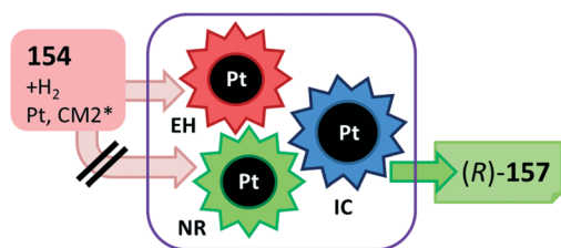
Scheme 46 Cascade EH, NR and IC of 2-nitrophenylpyruvates over chirally modified supported Pt catalyst. 203,204
