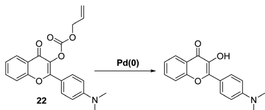
Scheme 21 Pd catalyzed decarboxylative deprotection of probe 22 , a process that allows for the ratiometric fluorescence detection of 0, +2 and +4 Pd species. Measurement conditions: PBS/THF (9 : 1) pH = 7.4.
