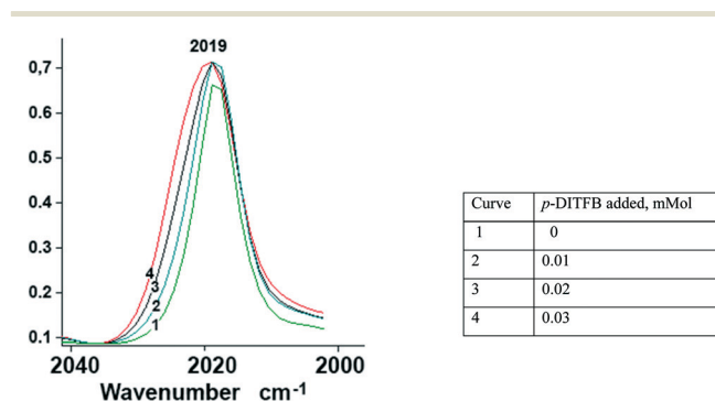
Fig. 1 Unsymmetrical hypsochromic broadening (ca. ~4 cm -1 half-width) of the \nu(\text{CO}) band at 2019 cm -1 as a result of gradual addition of p -DITFB to a 0.025 mmol cyclohexane solution of CpFe(CO) 2 TePh.
