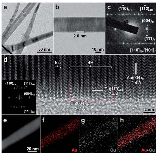
Fig. 4 (a) Low-magnification TEM image of alternating 4H/fcc bimetallic Au@Cu core-shell NRs. (b) High-magnification TEM image and (c) corresponding SAED pattern of a representative Au@Cu NR. (d) A representative HRTEM image of Au@Cu NRs. Inset: the corresponding FFT pattern of the selected region, i.e. the magenta dashed rectangle in (d). (e) HAADF-STEM image, and (f–h) corresponding STEM-EDS element maps of a representative Au@Cu NR.
