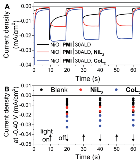
Fig. 6 (A) Current density measurements with three 10 s light on/off cycles with -0.40\text{ V} applied bias on a single \text{NiO}|\text{PMI}|30\text{ALD} working electrode without catalyst (black, "blank") and again after additional 0.5 mM \text{NiL}_2 (red) or 0.5 mM \text{CoL}_2 (blue). (B) Results of the same experiment with 5–30 cycles of \text{Al}_2\text{O}_3 ALD from Fig. S16.† The number of cycles of ALD is not distinguished for clarity (conditions: 0.1 M \text{H}_2\text{SO}_4 and 0.1 M \text{Na}_2\text{SO}_4 in 1 : 1 \text{H}_2\text{O} : MeCN).
