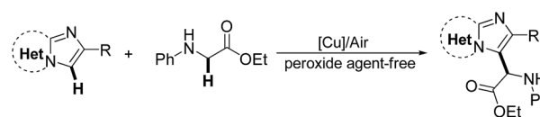
Scheme 1 Oxidative coupling of imidazoheterocycles with glycine esters.
