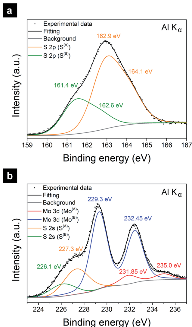
Fig. 2 Chemical analysis of the \text{MoS}_x /GCNT/CP electrode with XPS in (a) S 2p, and (b) Mo 3d–S 2s regions.
