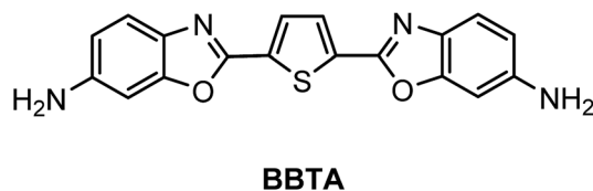
Scheme 1 Chemical structure BBTA.
