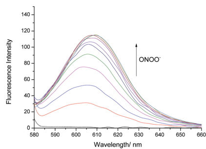
Fig. 2 Fluorescence spectra of TCFB2 (10 \mu\text{M} ) with addition of \text{ONOO}^- (0–10 \mu\text{M} ) in PBS buffer solution, 20% DMSO, pH 8.00 at 25 ^{\circ}\text{C} . \lambda_{\text{ex}} = 560 nm. Slit widths ex = 10 nm and em = 15 nm.
