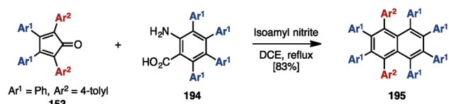
Scheme 37 [4+2] cycloaddition of tetraarylcylopentadienone and tetraarylbenzine.
