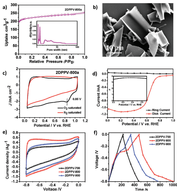
Fig. 3 (a) Nitrogen adsorption–desorption isotherms of 2DPPV-800a (inset: pore size distribution); (b) SEM image of 2DPPV-700; (c) CV curves of 2DPPV-800a in N_2 -saturated and O_2 -saturated 0.1 M KOH at a scan rate of 50\text{ mV s}^{-1} ; (d) RRDE voltammogram for 2DPPV-800a in 0.1 M KOH solution saturated with O_2 (the electrode rotation rate was 1600 rpm and the Pt ring electrode was held at 0.5 V, inset: electron transfer number of 2DPPV-800a as a function of potential); (e) CV curves of 2DPPV-X ( X = 700, 800, 900 ) at 5\text{ mV s}^{-1} in 6 M KOH aqueous solution; and (f) galvanostatic charge/discharge curves for 2DPPV-X ( X = 700, 800, 900 ) at a current density of 0.5\text{ Ag}^{-1} .
