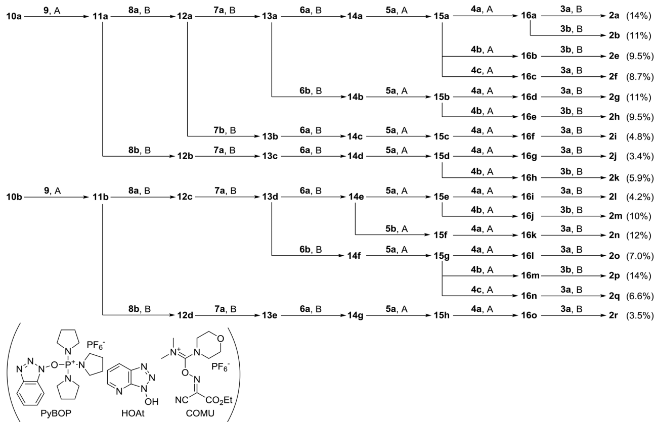
Scheme 1 Syntheses of the analogues 2a, 2b, and 2e-r. Overall yields from 9 are given in parentheses. Reagents and conditions: (A) (i) TFA, CH 2 Cl 2 , (ii) PyBOP, HOAt, i -Pr 2 NEt, DMF; (B) (i) TFA, CH 2 Cl 2 , (ii) COMU, 2,4,6-collidine, DMF. COMU = (1-cyano-2-ethoxy-2-oxoethylidenaminoxy)dimethyl-amino-morpholino-carbenium hexafluorophosphate; DMF = N,N -dimethylformamide; HOAt = 1-hydroxy-7-azabenzotriazole; PyBOP = benzotriazol-1-yl-oxytripyrrolidinophosphonium hexafluorophosphate; TFA = trifluoroacetic acid.
