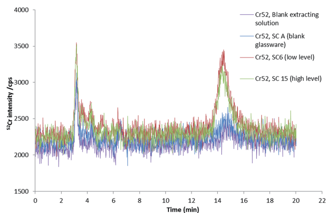
Fig. 6 HPLC-ICP-MS chromatogram of Cr species in mainstream smoke from cigarette spiked two different spike levels (5.80 and 9.80 \mu\text{g g}^{-1} of chromium, respectively) using 2.8 mM TPABr and 4 mM EDTA (pH 8.5) as extractant. 0.18 mM, 1 mM EDTA (pH 8) as mobile phase at a flow rate of 0.8 mL min -1 .
