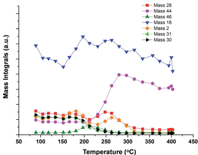
Fig. 7 TPPR (temperature-programmed pulsed reaction) profiles for methanol pulses into a flow of He.
