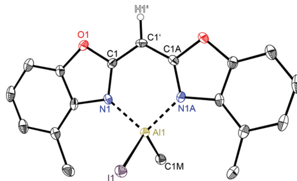
Fig. 8 Molecular structure of [\text{IMeAl}\{(4\text{-MeNCOC}_6\text{H}_3)_2\text{CH}\}] (6). Anisotropic displacement parameters are depicted at the 50% probability level. C–H hydrogen atoms are omitted for clarity except for the one at the bridging CH group. Structural data are given in Tables 1–3.
