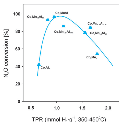
Fig. 8 Dependence of \text{N}_2\text{O} conversion on the amount of reducible components in the interval of 350–450 °C. Reaction conditions: 0.1% \text{N}_2\text{O} , He balance; total flow rate = 100 ml \text{min}^{-1} ; mass of catalyst = 100 mg; temperature = 450 °C (adapted from ref. 169 with kind permission from Elsevier).
