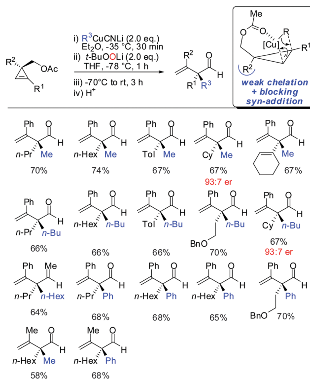
Scheme 38 Carbometallation-oxidation-elimination sequence.
