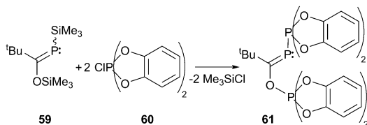
Scheme 23 Condensation of silylated phosphoalkene 59 and chlorophosphorane 60 giving 61 , which features the rare \sigma^2 - \sigma^5 bonding motif G .
