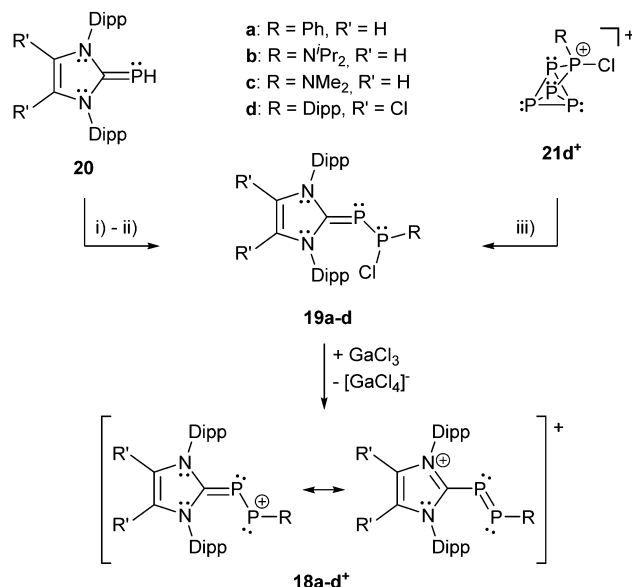
Scheme 7 Two different approaches for the synthesis of NHC stabilized chlorodiphosphenes 19a-d comprising bonding motif B. For 19a,b : (i) + \text{R}(\text{P}(\text{Cl})\text{R})_2 , + DABCO, -\text{DABCO}\cdot\text{HCl} ; for 19c : (ii) + 2\text{PCl}(\text{NMe}_2)_2 , + DABCO, -\text{DABCO}\cdot\text{HCl} , -\text{P}(\text{NMe}_2)_3 ; for 19d : (iii) + 3 1,3-bis(2,6-diisopropylphenyl)-4,5-dichloro-imidazole-2-ylidene, -\text{5}^+ . Subsequent chloride abstraction yields polarized cationic diphosphenes 18a-d + . Only two resonance structures that indicate the polarization of 18a-d + are shown.
