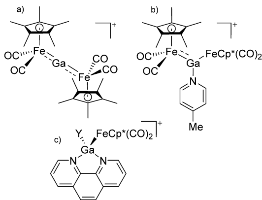
Fig. 22 (a) The linear di-coordinated cation [(FP^*)_2(\mu-Ga)]^+ derives from a salt metathesis of (FP^*)_2GaCl and Na^+[B(Ar^{CF_3})_4]^- . The Fe–Ga–Fe moiety features a significant \pi bonding component (population analysis). 169 (b) The [(FP^*)_2(\mu-Ga)-(4-Pic)]^+ cation is an addition product of [(FP^*)_2Ga]^+ and 4-Pic and the second structurally characterized complex containing a cationic tricoordinate gallium centre. 170 (c) Applying the chelating phen ligand, Ueno et al. isolated the tetra-coordinated [(FP^*)Ga(phen)(Y)]^+ ( Y = Cl, S^2Tol ) cations, i.e. the first transition-metal complex with a thiolate group on the gallium atom. 171
