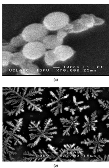
Fig. 19 SEM images of \text{Ga}_2\text{O}_3 deposited at 550 °C from [\text{Ga}(\text{NMe}_2)_3]_2 with (a) \text{HOCH}(\text{CH}_2\text{NMe}_2)_2 and (b) \text{HOCH}(\text{CH}_3)\text{CH}_2\text{NMe}_2 in toluene. Reproduced from ref. 154 with permission from The Royal Society of Chemistry.
