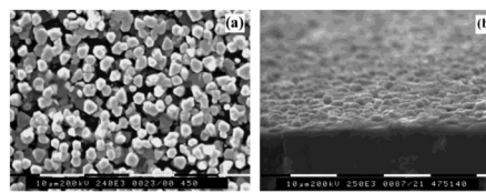
Fig. 33 SEM images of \text{Bi}_2\text{Se}_3 deposited from [\text{Bi}(\text{N}(\text{Se}^i\text{Pr}_2)_2)_3] by AACVD at 475 °C on glass. Reproduced with permission from ref. 116. Copyright 2004 Copyright 2013 American Chemical Society.
