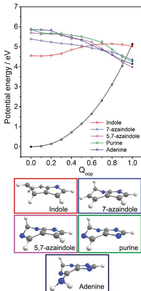
Fig. 13 Overlaid diabatic PECs along Q_{oop} for the 1^1\pi\pi^*/S_0 state that correlates with the 1^1\pi\pi^*/S_0 MECI in indole, 7-azaindole, 5,7-azaindole, purine and A. The filled points show the energies of the optimised critical structures (i.e. the S_0 state minimum and the S_0/1^1\pi\pi^* MECI) and, for clarity, only the S_0 PEC calculated for indole is shown (open black points). The optimised geometry at each MECI is shown below.
