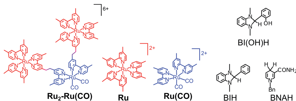
Chart 1 Structures and abbreviations of \text{Ru}_2\text{-Ru(CO)} , model mononuclear complexes, \text{BI(OH)H} , \text{BIH} , and \text{BNAH} . The counter anions of the complexes were \text{PF}_6^- .
