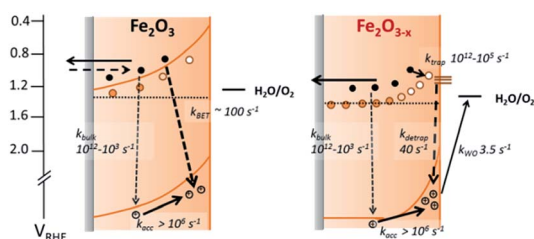
Scheme 1 Simplified energy diagrams and processes involving photo-generated charges following UV laser excitation of \alpha -Fe _2 O _3 and \alpha -Fe _2 O _{3-x} under a positive bias. Rate constants are those determined at 1.4 V_{\text{RHE}} as described in the main text. In contrast to \alpha -Fe _2 O _3 which has been air annealed, no slow recombination between surface accumulated holes and bulk electrons ( k_{\text{BET}} ) is observed for \alpha -Fe _2 O _{3-x} .
