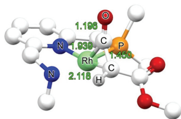
Fig. 3 DFT optimized structure of \text{NINT3} (bond lengths in Å).
