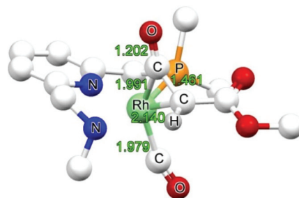
Fig. 4 DFT optimized structure of \text{NINT6} (bond lengths in Å).
