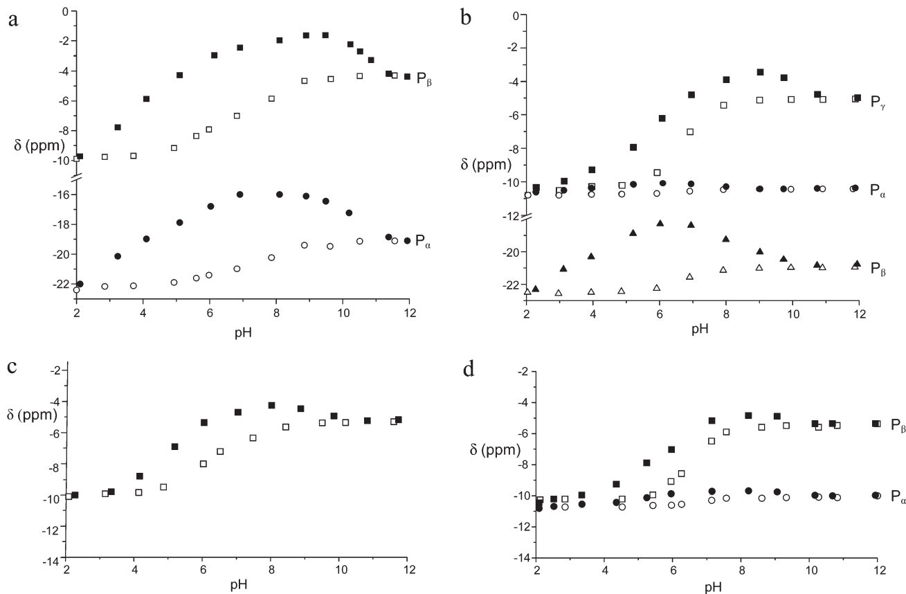
Fig. 6 pH dependence of the ^{31}\text{P} NMR signals (162 MHz) of (a) TP, (b) ATP, (c) PP, and (d) ADP in the presence (filled symbols) and in the absence (empty symbols) of the \text{Zn(II)} complex of 1 . Conditions: [\mathbf{1}] = [\text{Zn}^{2+}] = [\text{TP}] = [\text{PP}] = [\text{ADP}] = [\text{ATP}] = 5 \times 10^{-3} \text{ M} , 308 K.
