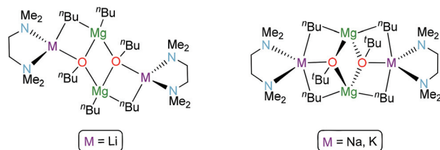
Fig. 5 ChemDraw representations for [(TMEDA)LiMg( n Bu) 2 (O n Bu)] 2 (5) (left) and Mulvey's alkali metal alkoxide–magnesium bis(alkyl) dimers (inverse crowns) [(TMEDA)MMg( n Bu) 2 (O n Bu)] 2 , M = Na, K (right).
