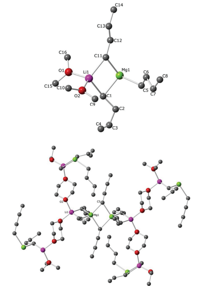
Fig. 6 Molecular structure of 6, showing asymmetric unit; (top) and polymer propagation (bottom). All hydrogen atoms are omitted for clarity.
